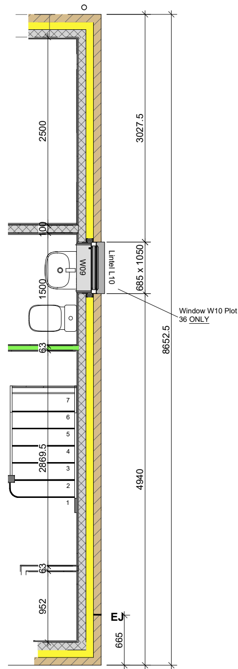
2 Ground Floor - Plot 36 Callout 1 : 50
